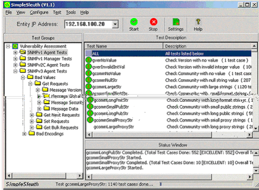
Fig1: Screen shot of the SimpleSleuth running SNMPv1 Agent Tests.
